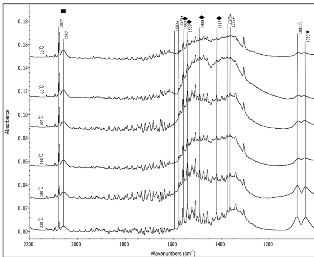
Fig. 5. In situ IR spectra for methanol synthesis from \text{CO}_2/\text{H}_2 recorded during temperature-programmed-reaction at low wave number area. \text{HCOO-Zn} (●), carbonate (◆), \text{CH}_3\text{O-Zn} (☆), \text{CH}_3\text{OH} (★).
