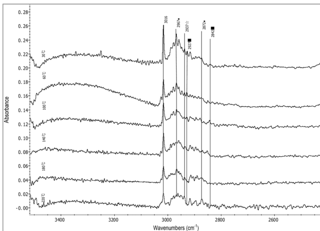
Fig. 4. In situ IR spectra for methanol synthesis from \text{CO}_2/\text{H}_2 recorded during temperature-programmed-reaction at high wave number area. \text{HCOO-Zn} (●), \text{CH}_3\text{O-Zn} (☆), \text{HCOO-Cu} (■).
